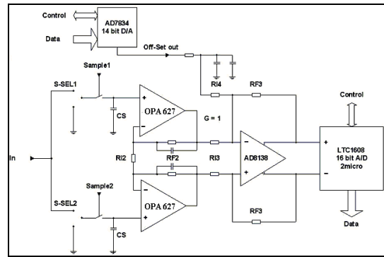
Figure 3. Signal Processing (one channel)
