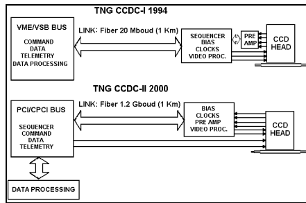
Figure 1. Block Diagram of the two CCD controller
