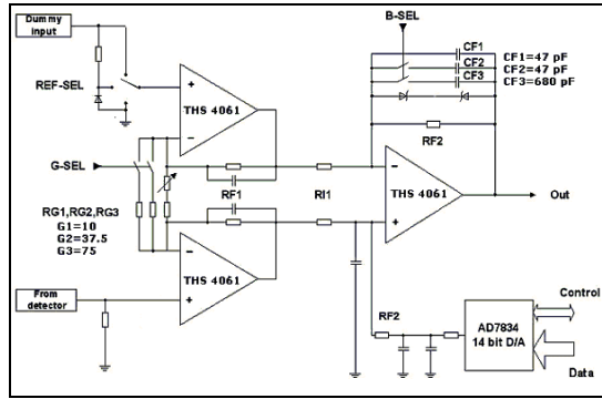
Figure 2. Preamplifier (one channel)
